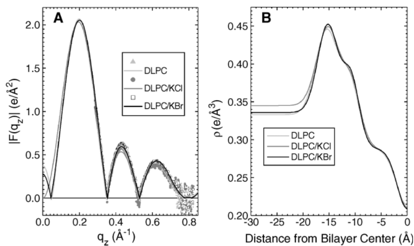
Fig. 4. A: Absolute values of continuous form factors: symbols are data and lines are model fit to the data. Negative values indicate statistical fluctuations when the form factors are close to zero. B: Electron density profiles of DLPC, DLPC/1 M (bulk) KCl, and DLPC/0.1 M (bulk) KBr at 30°C. Half of the bilayer is shown. Note the difference in electron densities of the different solvents that accounts for most of the differences in the form factors in A.
